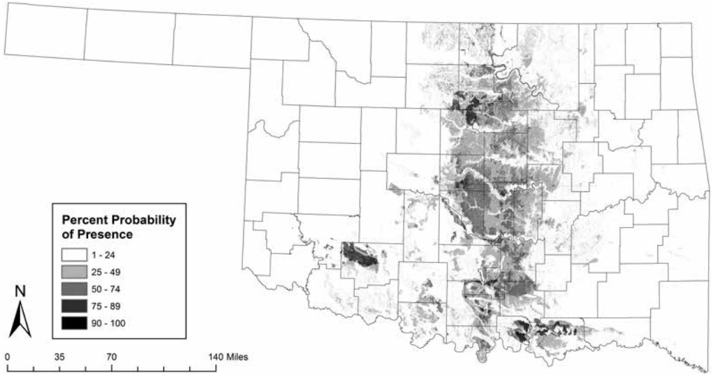
Fig. 3. Prediction map for Penstemon oklahomensis potential distribution within Oklahoma; Model 20 B.
